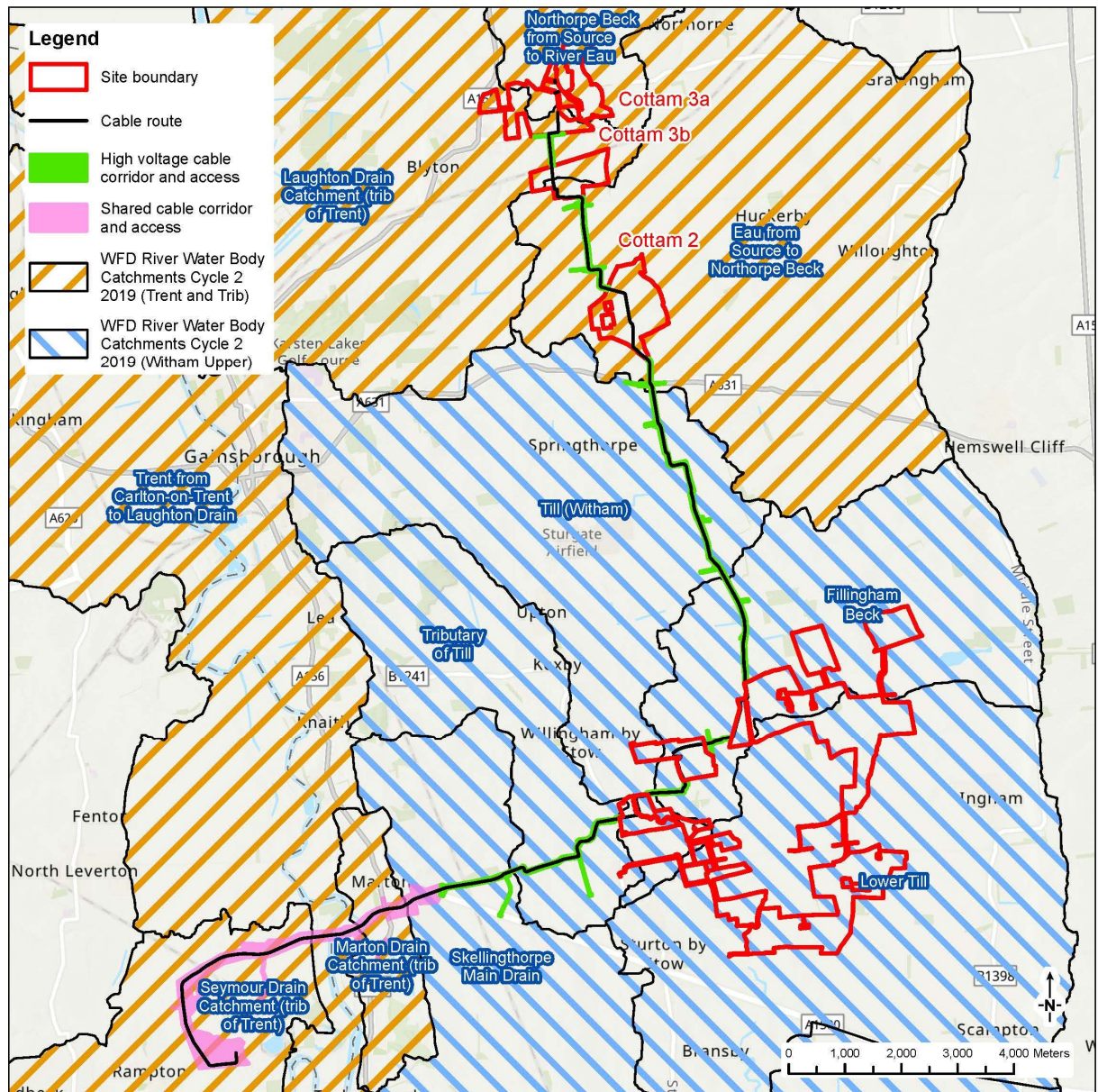
Figure 2: Waterbody Catchments
